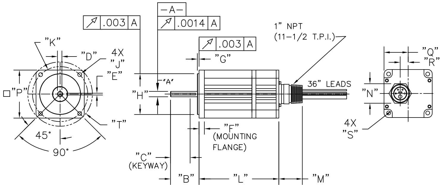
M43X "SX" OUTLINE
