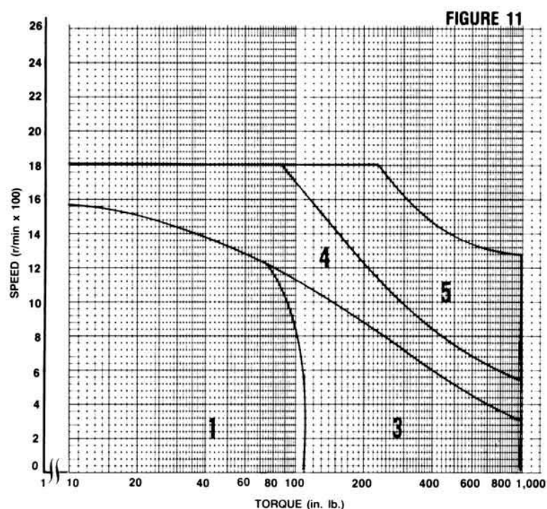
D.C. OPERATION FOR M134, M234 MOTOR
