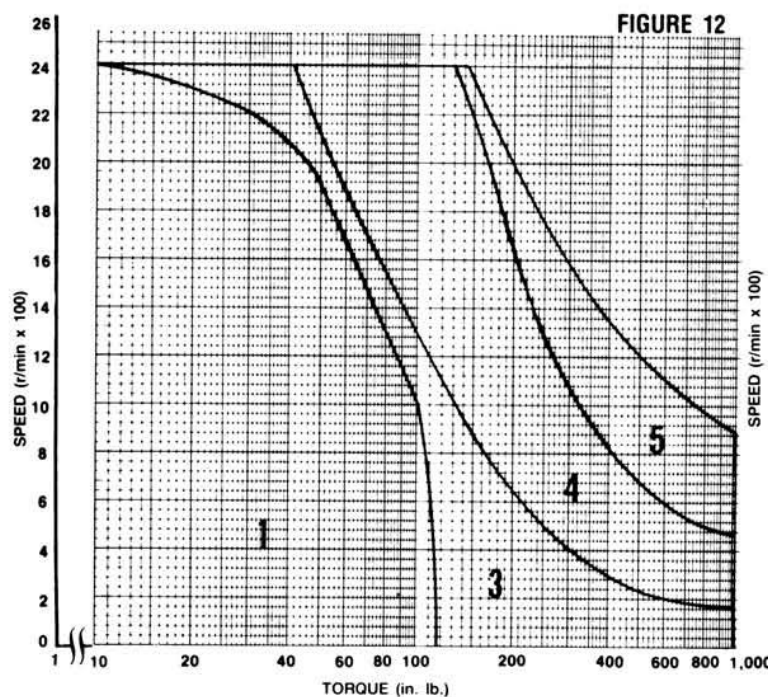
D.C. OPERATION FOR M133, M233 MOTOR
