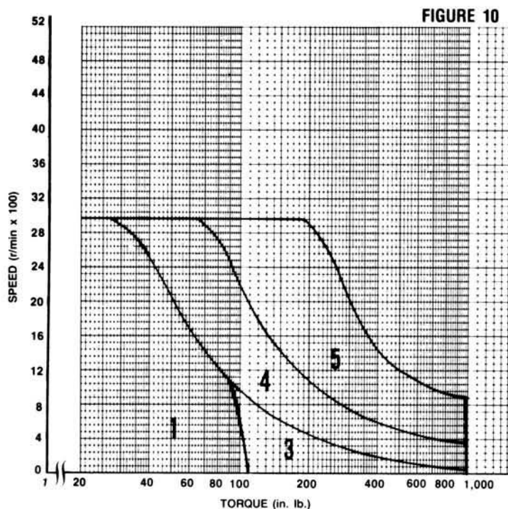
D.C. OPERATION FOR M133, M233 MOTOR
