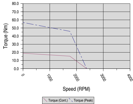
SW & SF-Series: M473-C Winding
