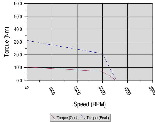
SX-Series: M462-G Winding
