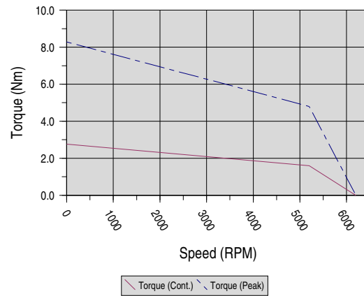
SW & SF-Series: M432-N Winding
