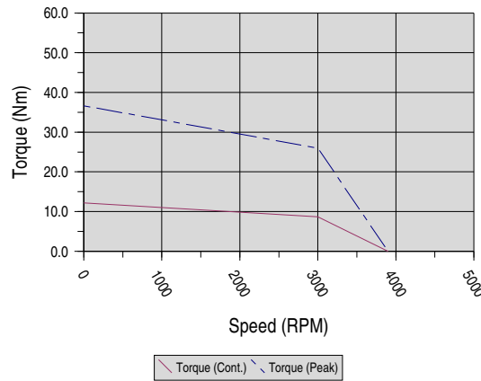
SW & SF-Series: M462-G Winding
