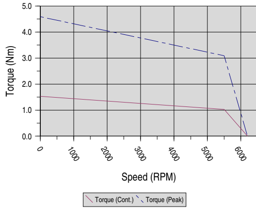
SW & SF-Series: M431-N Winding
